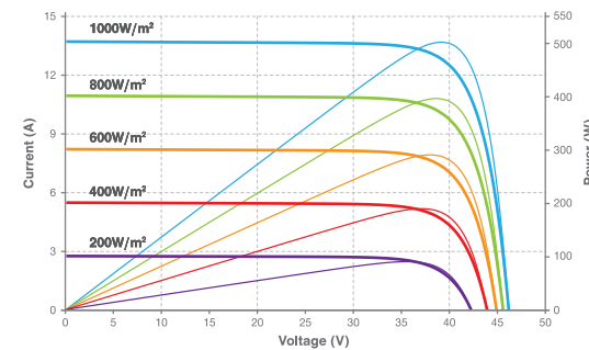
Current-Voltage & Power-Voltage Curve (500W)
