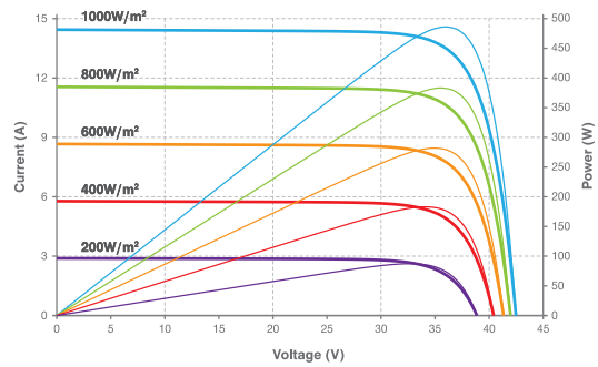
Current-Voltage & Power-Voltage Curve (485W)
