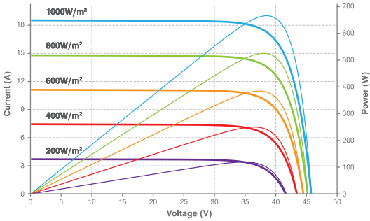
Current-Voltage & Power-Voltage Curve (665W)
