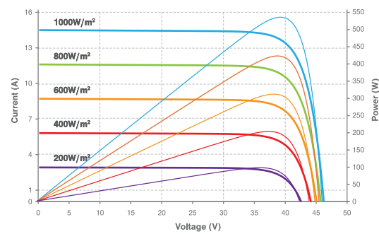
Current-Voltage & Power-Voltage Curve (535W)
