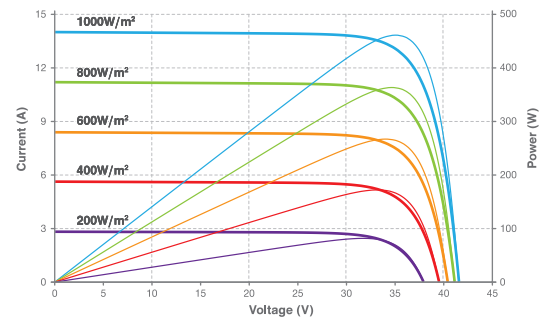
Current-Voltage & Power-Voltage Curve (460W)
