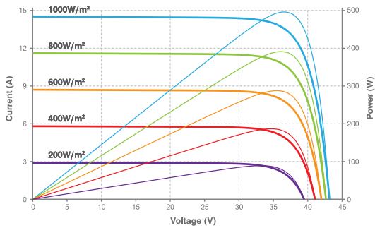
Current-Voltage & Power-Voltage Curve (495W)
