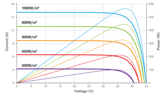
Current-Voltage & Power-Voltage Curve (565W)
