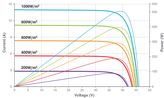
Current-Voltage & Power-Voltage Curve (505W)
