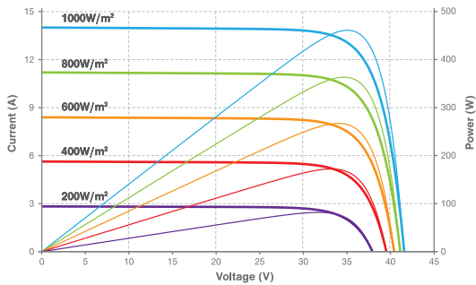
Current-Voltage & Power-Voltage Curve (460W)
