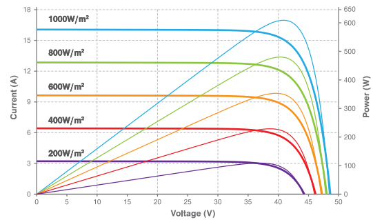
Current-Voltage & Power-Voltage Curve (615W)
