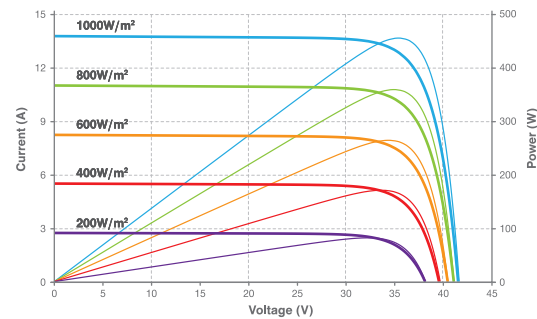
Current-Voltage & Power-Voltage Curve (455W)
