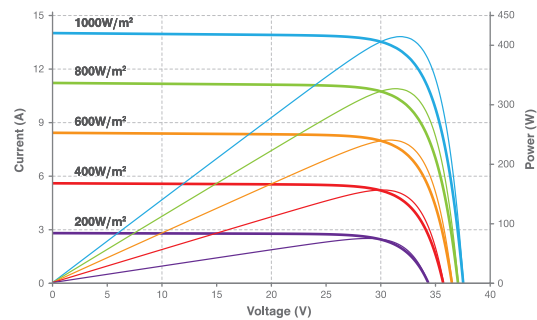
Current-Voltage & Power-Voltage Curve (415W)
