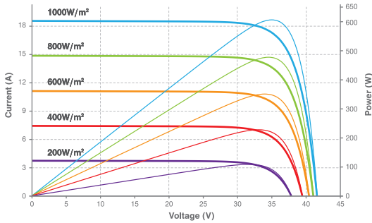
Current-Voltage & Power-Voltage Curve (605W)
