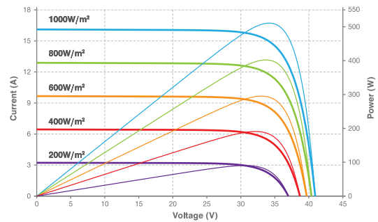
Current-Voltage & Power-Voltage Curve (510W)
