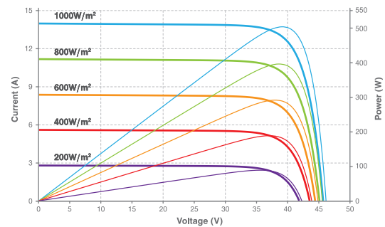
Current-Voltage & Power-Voltage Curve (505W)
