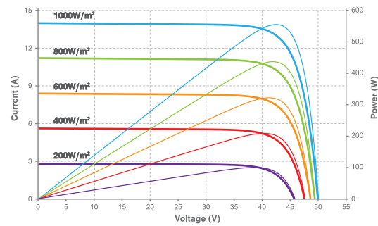
Current-Voltage & Power-Voltage Curve (555W)
