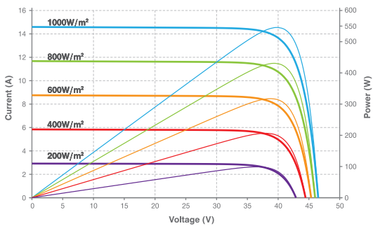
Current-Voltage & Power-Voltage Curve (545W)
