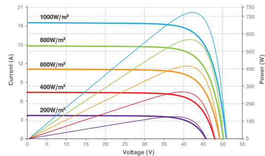
Current-Voltage & Power-Voltage Curve (720W)
